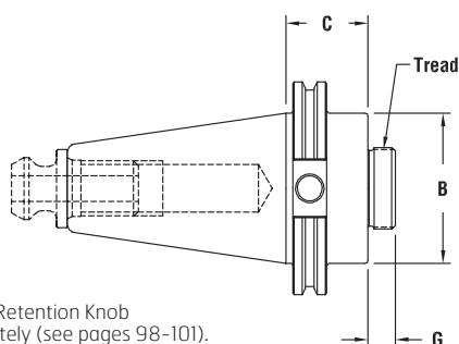
Boring Head Holder C40-62BH1 shown here.
